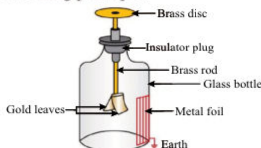
Fig: 14.8 Schematic diagram of electroscope
