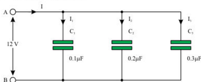
Fig: 14.19 Parallel combination of three capacitors
