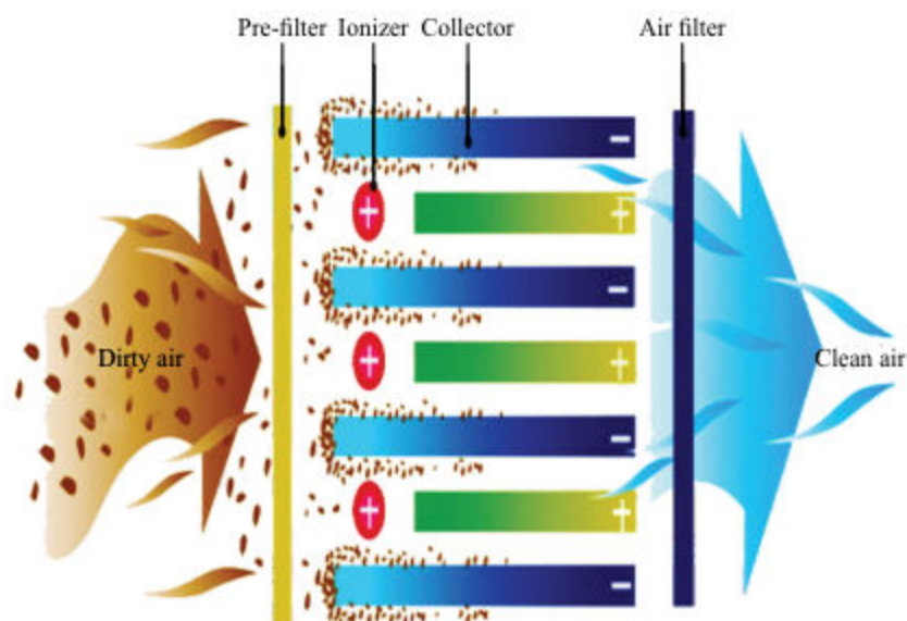
Fig: 14.15 Systematic diagram of electrostatic air cleansing
